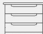
3-Drawer Chest H:685mmxW:780mmxD:545mm INDI-3DRCHEST
