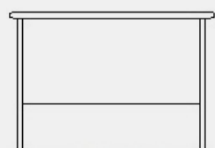
Open Desk H:745mmxW:1000mmxD:500mm INDI-Desk
