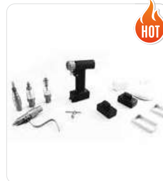
MSLGK14 Vet Orthopedic Drill And Saw
